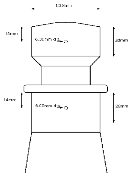
図5 Pylon Specification Drawing
