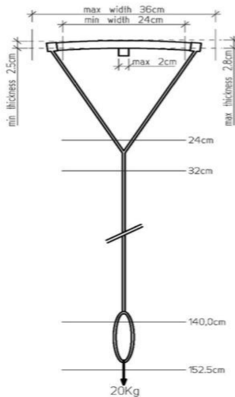
Diagram 9 - Handle measurement device dimensions
